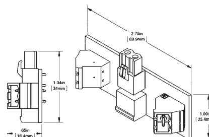
BA/BP-BR - Power Bridge
