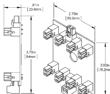
BP4-V - Vertical Backplane
