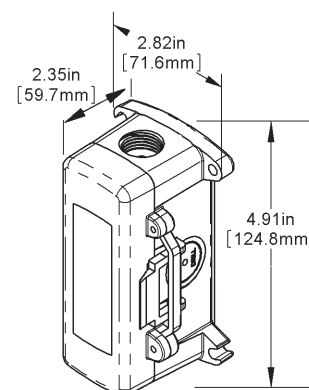
XOR-BB2 Model
