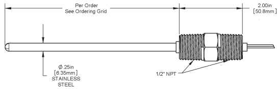
Probe without Enclosure
