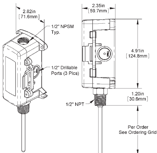
BAPI-Box 2 "Outside Mount" (BB2O)
