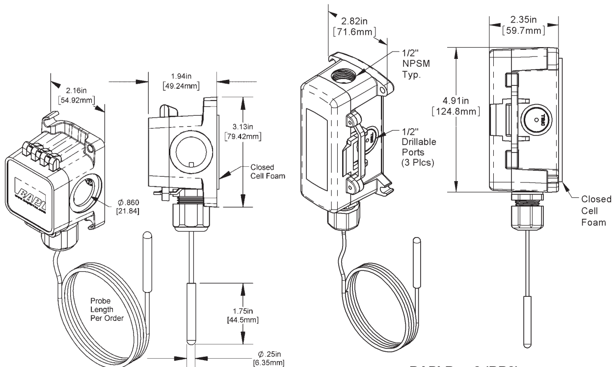
BAPI-Box 2 (BB2)
