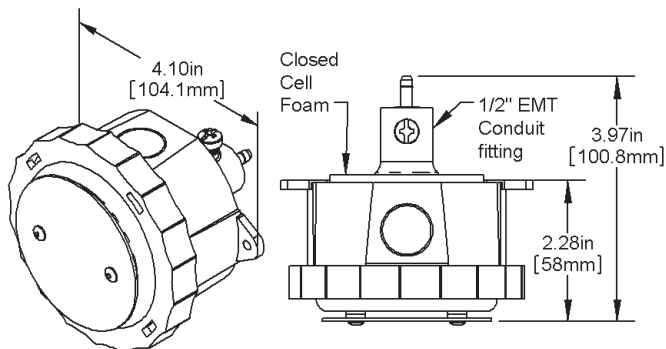
Vertical Mount
