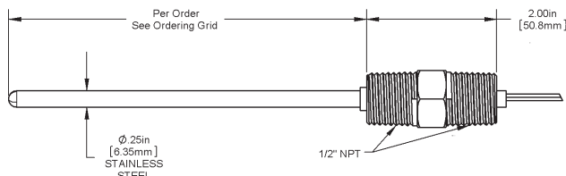
Immersion Probe without Enclosure
