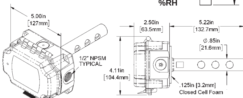
Duct Mount (Dimensions are the same for the rough service unit without the aspiration tube)
