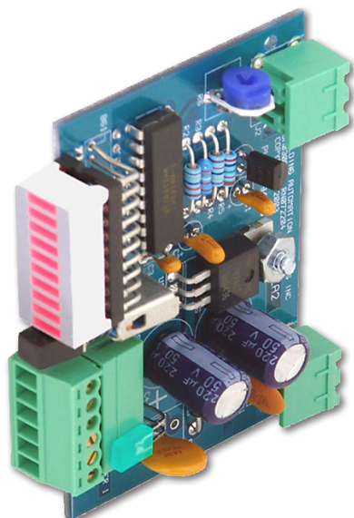
EA2 - Modulating Actuator Interface (p. H6)
