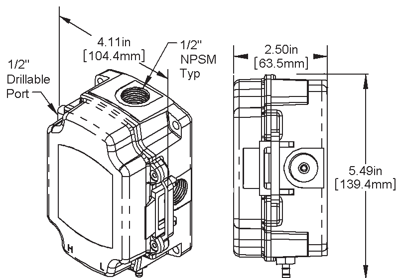
BAPI-Box Enclosure Units
