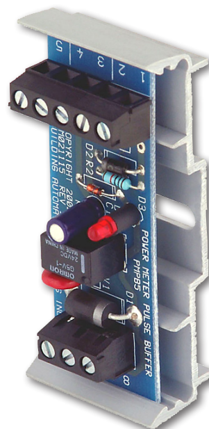
PMPB5 mounted in optional 2.75" snaptrack
