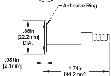
Low Profile Port
