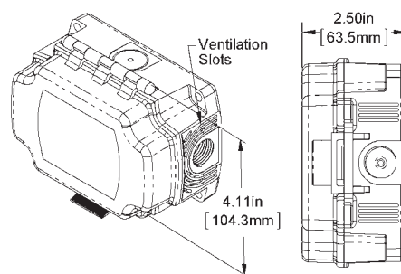
CO 2 Rough Service Sensor
