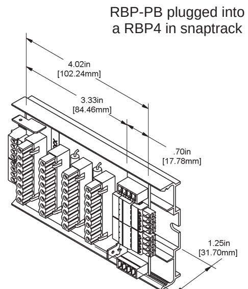
RBP-PB Power Bridge
