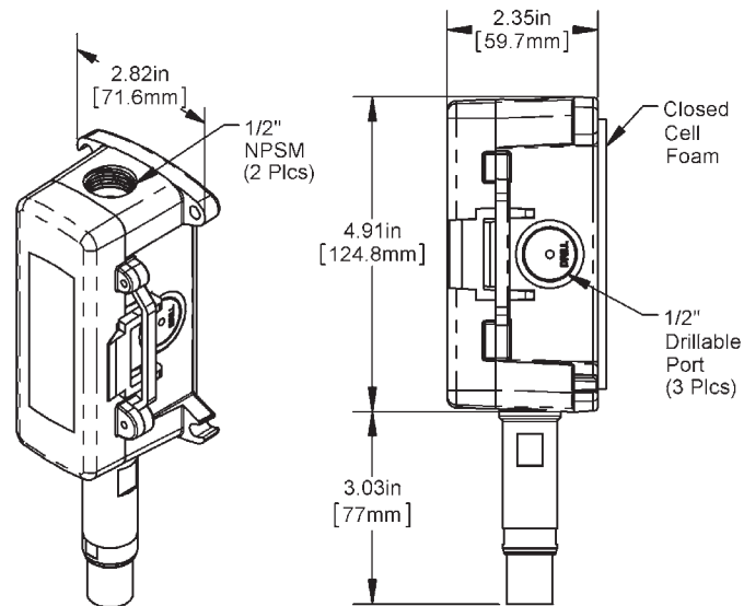
BAPI-Box 2 (BB2)
