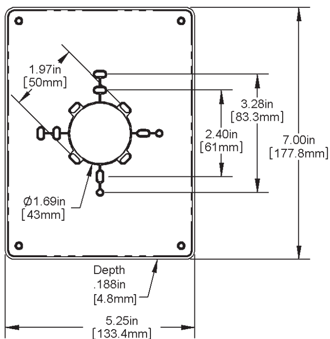
BA/ADP-525-7-BW
