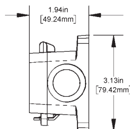
-STM Model (shown with optional Terminal Strip)
