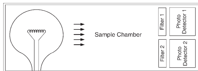
Fig. 2: Dual Channel CO 2 Sensor
