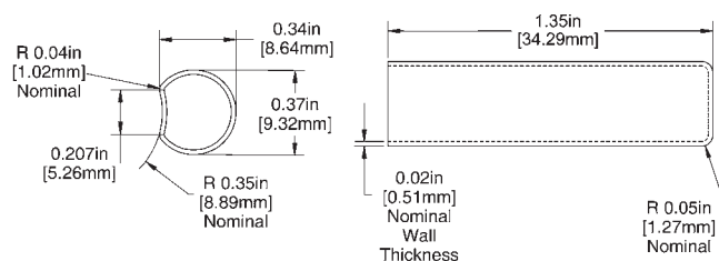
Concave Probe
