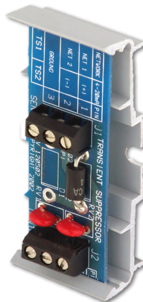
TS1 or TS2 Transient Suppressor with optional 2.75" snaptrack
